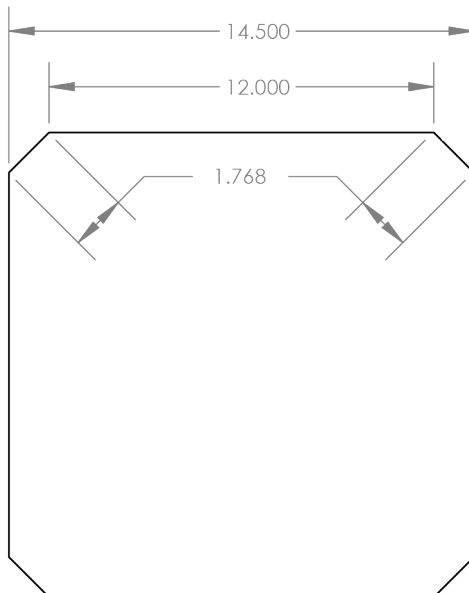
SNK-15D / SSNK-15D ISLAND TOP VIEW CUTOUT DIMENSIONS
